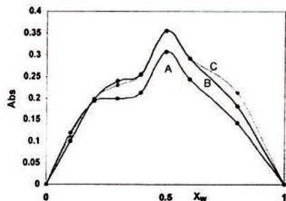
Figure 1. Continuous-variation plots of the absorbances of \text{WO}_3\text{L}^{3-} , abs, vs the mole fraction of \text{W(VI)} , X_w , at 25^\circ\text{C} , an ionic strength of 0.1 \text{ mol dm}^{-3} \text{NaClO}_4 , and different wavelengths: A, 260 nm; B, 265 nm; and C, 270 nm.
